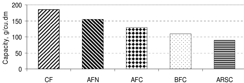
Figure 2. Dust capacity of fluted and Direct Flow Filters, CF - Direct Flow filter, HD cellulose filter media, AFN company A, commercial fluted filter, nanofiber filter media, company A, commercial fluted filter, cellulose filter media, BFC - company B, commercial fluted filter, Cellulose filter media, ARSC - company A, commercial radial seal cylindrical filter
