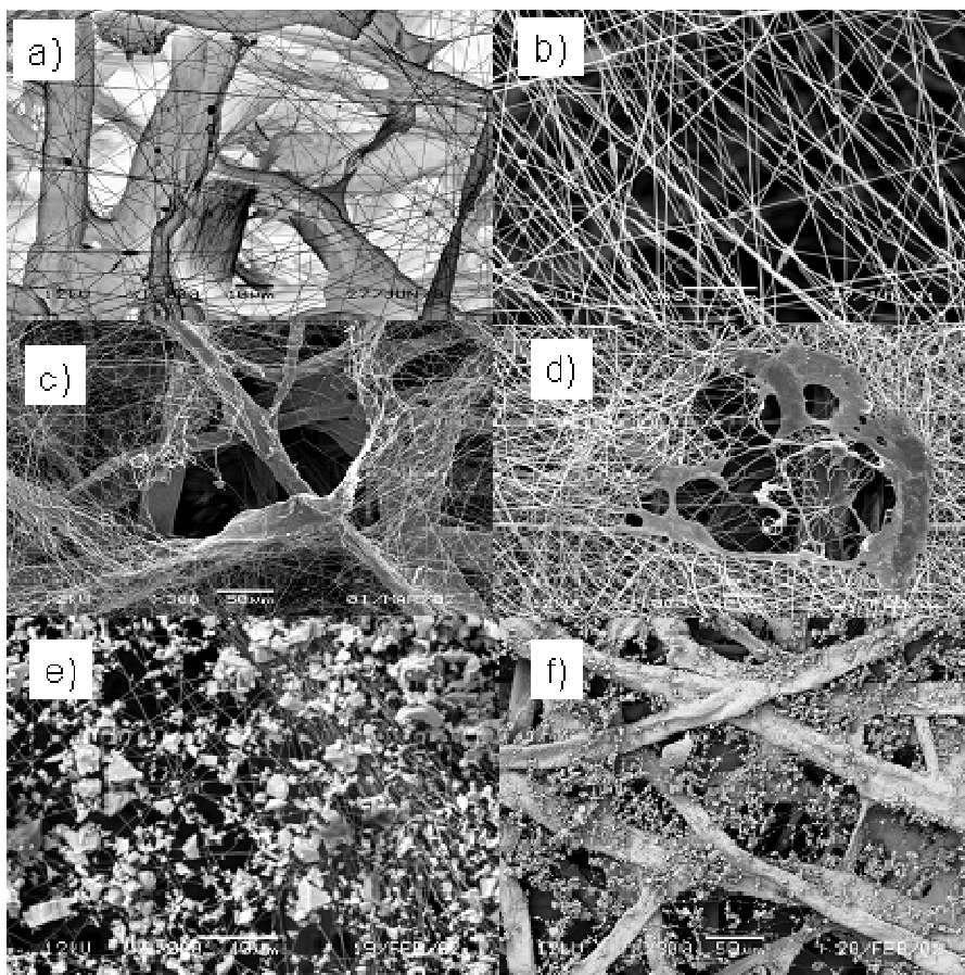
Figure 4. Uniform (a and b) and non-uniform (c and d) nanofiber and dust cake distribution (e and f).
