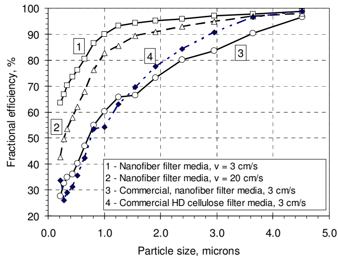
Figure 3. Fractional efficiency of pleatable filter media.
