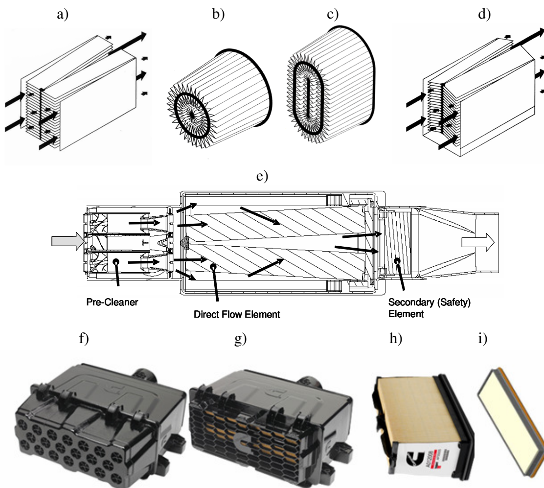
Fig. 1. Schematic and full view of Direct Flow filters; a) flow pattern through a rectangular filter with 2- filter elements, b) multi cylindrical filter, c) elliptical multi element filter ,d) filter element with skewed pleats, e) schematic view of filter assembly, f) Direct Flow filter with through flow cyclonic precleaner, g) Direct Flow filter with inlet grate, h) filter element, i) secondary (safety) filter .
